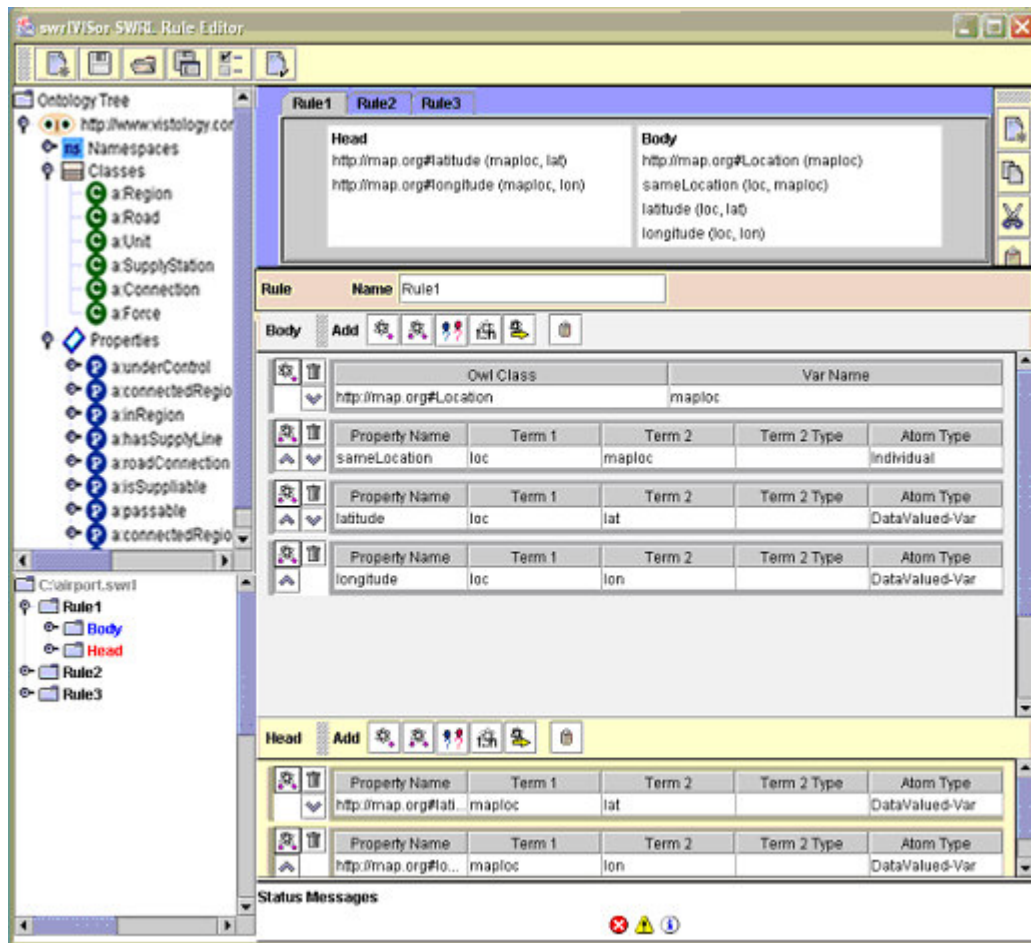
Figure 2. Screenshot depicting the appearance of SWRLeD, a graphical editor for SWRL rules.
