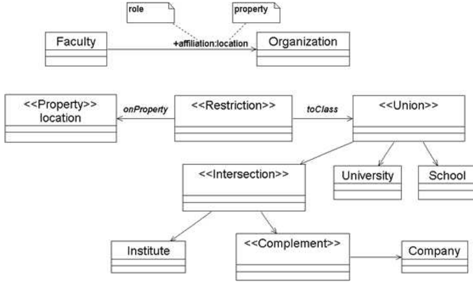
Fig. 11. Example Model using the Proposed UML Extension
