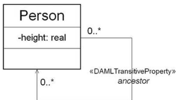
Fig. 8. Example of a Transitive Property
