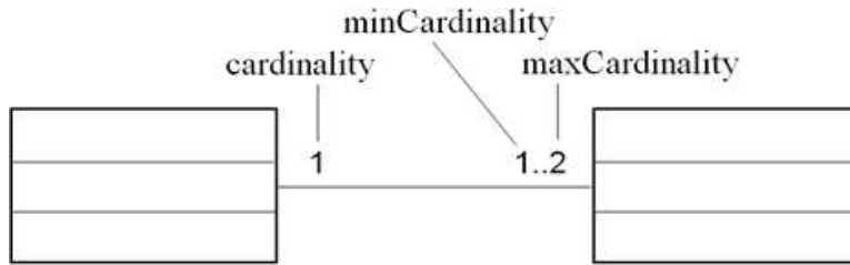
Fig. 6. DAML+OIL Cardinality
