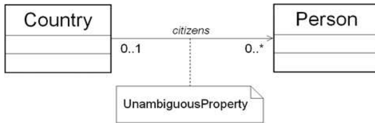
Fig. 7. Example of an Unambiguous Property
