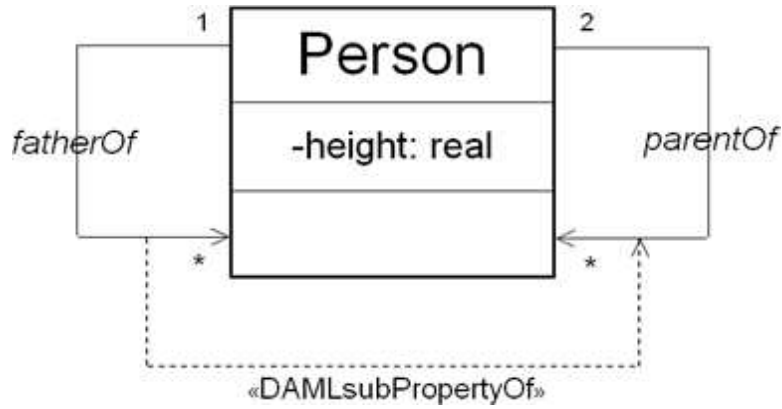
Fig. 4. Example of a SubProperty
