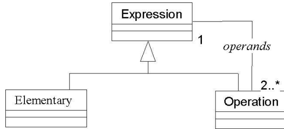
Fig. 2. Expression/Operation Ontology
